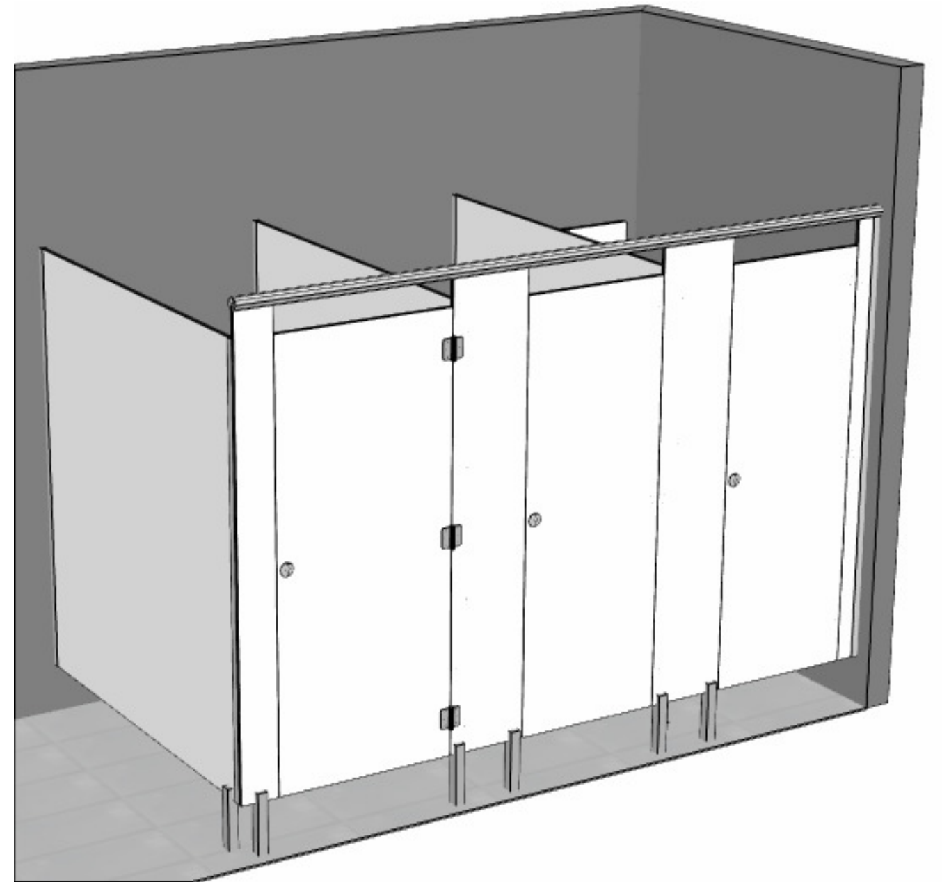
Perspective View
