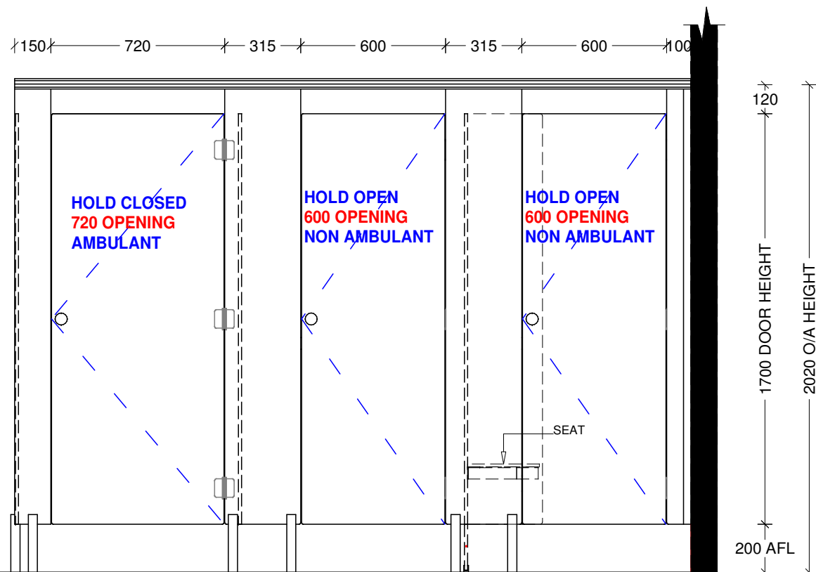
Elevation View
