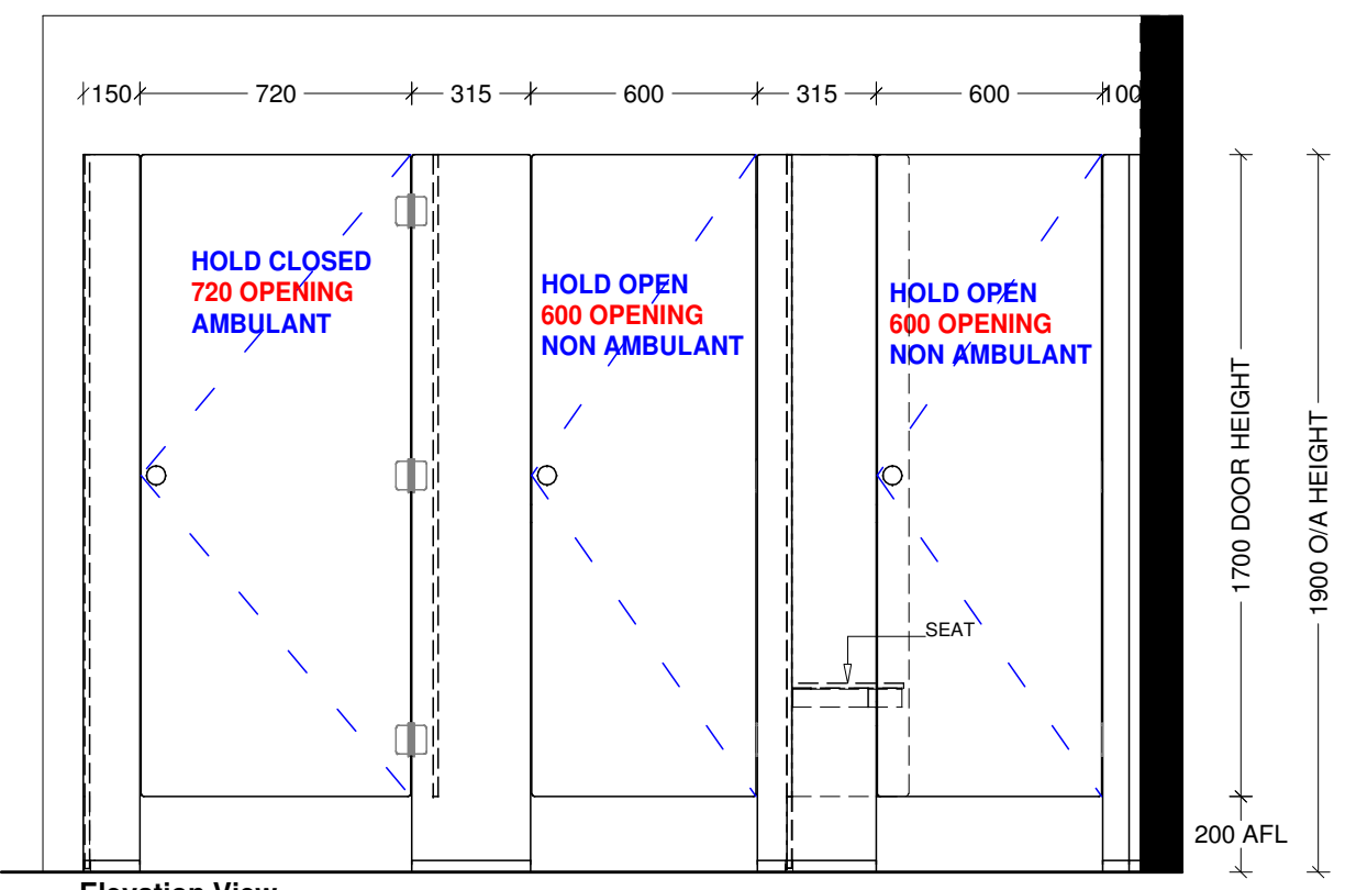
Elevation View
